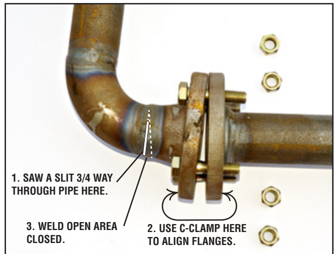
Figure 5. Flanges have unacceptable closed angle alignment.
