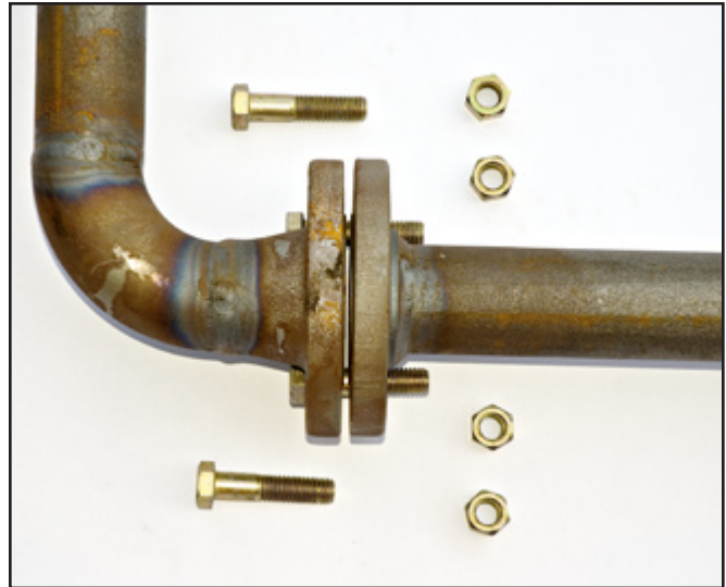
Figure 4. Flanges properly positioned before bolting.
