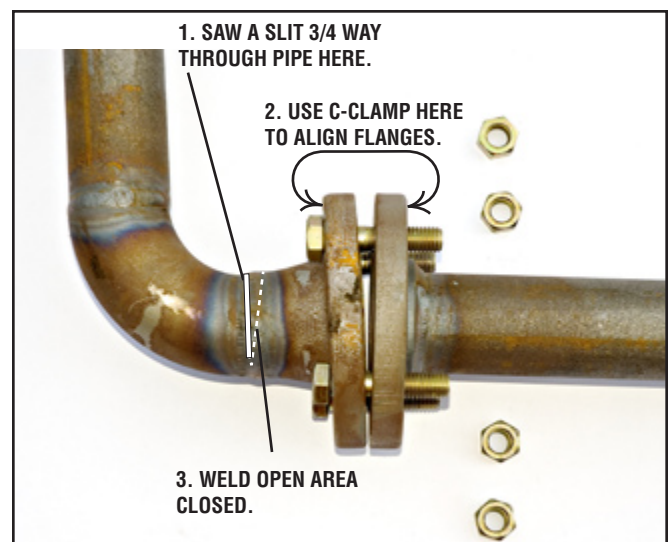
Figure 6. Flanges have unacceptable open angle alignment
