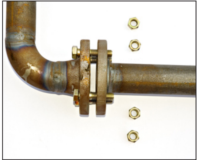
Figure 7. Flanges have too large a gap between them
