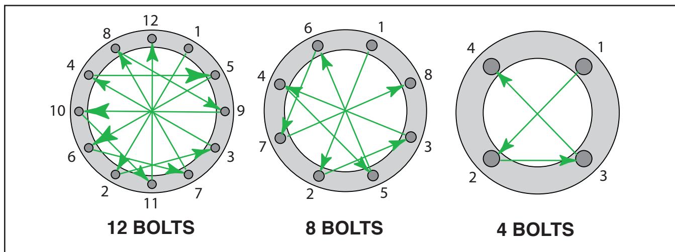
Figure 13. Tightening patterns.
