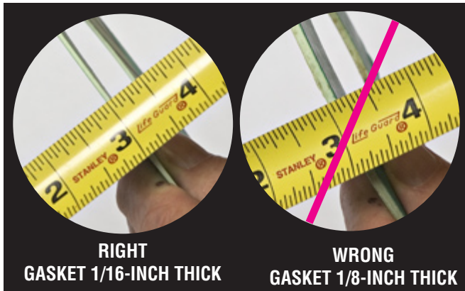
Figure 9. Right and wrong gaskets.
