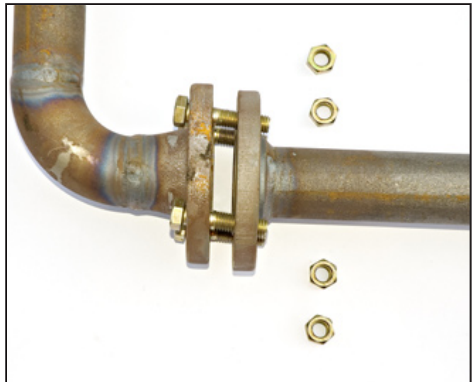
Figure 8. Flanges have unacceptable offset from each other.
